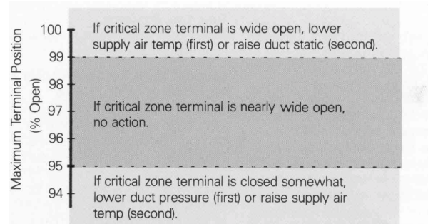
Figure 8. Operating Logic for Critical Zone Reset
