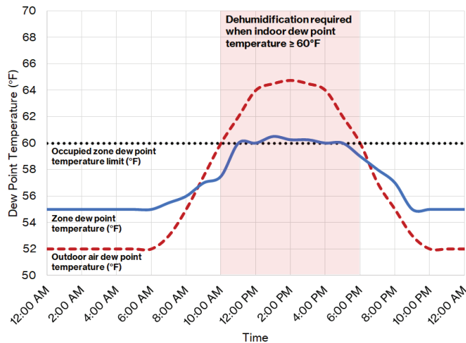
Figure 2. Example zone humidity when dehumidification is required
