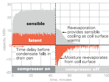
Figure 5. Part-load dehumidification (cycling compressor, constant-volume fan)
