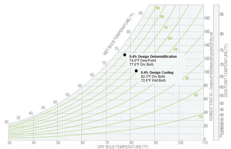
Figure 7. Hilo, Hawaii design cooling and design dehumidification weather conditions
