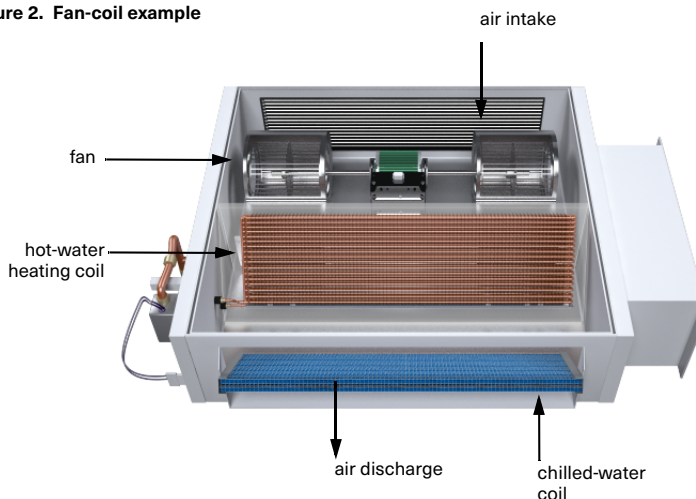
Figure 2. Fan-coil example
