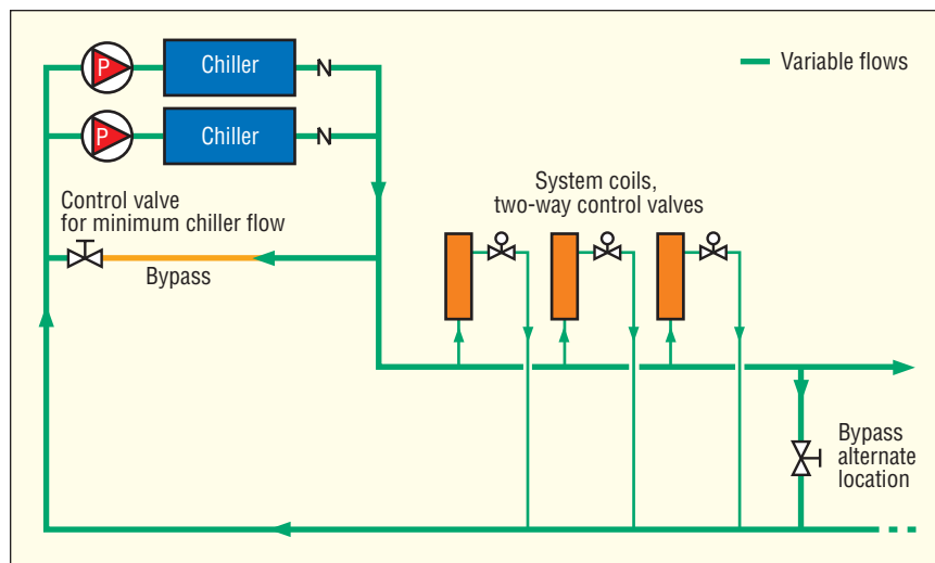
FIGURE 2. Variable primary-variable secondary flow system.
