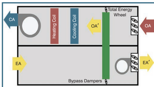
Figure 1: Exhaust-air energy recovery in a dedicated OA system.
