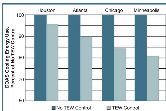
Figure 11: Annual DOAS cooling energy impact of proper total-energy wheel control.
