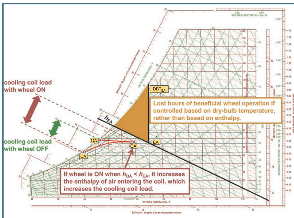
Figure 2: Total energy wheel control on a mild, rainy day.
