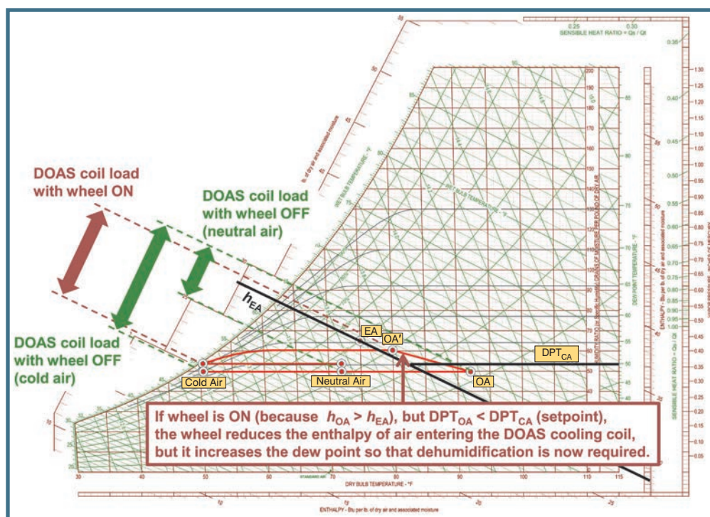
Figure 5: Total energy wheel control on a hot, dry day.
