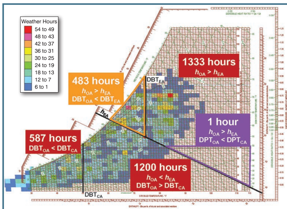
Figure 3: Distribution of total energy wheel operating hours (Atlanta). Monday through Friday 6 a.m. to 6 p.m.
