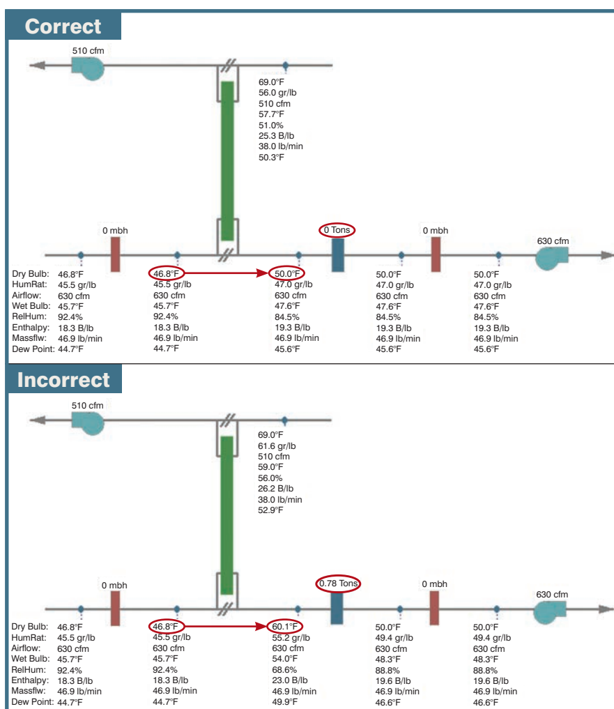
Figure 10: Modeling modulating capacity control on a cool day. Correct (top): When it is cool outside, wheel capacity should be modulated to avoid overheating, and it is. Wheel recovers only enough heat to warm the OA to 50°F (10°C) (winter setpoint). Incorrect (bottom): When it is cool outside, wheel capacity should be modulated to avoid overheating, but instead the wheel is operating at full capacity. The result is recovery of too much heat, warming the air above 50°F (10°C) (winter setpoint), which may require re-cooling.
