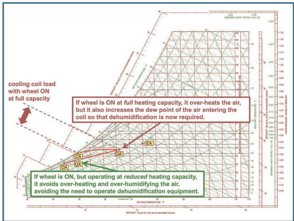
Figure 6: Total energy wheel control on a cool, dry day.
