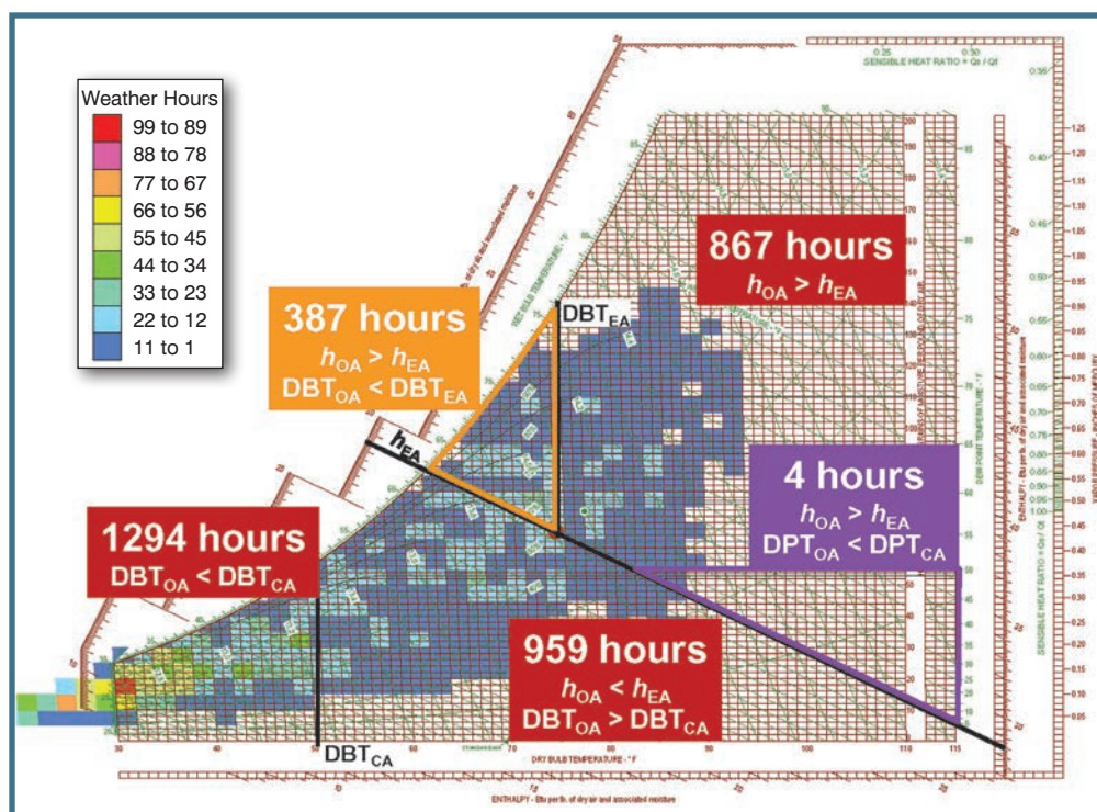
Figure 4: Distribution of total energy wheel operating hours (Chicago). Monday through Friday 6 a.m. to 6 p.m.
