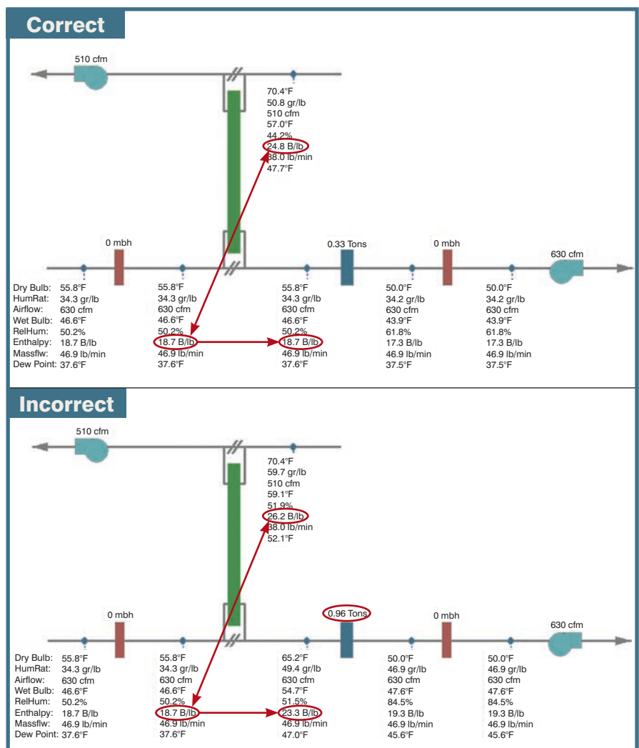
Figure 9: Modeling on/off total energy wheel control on a mild day. Correct (top): When h_{OA} < h_{EA} the wheel should be off, and it is off. Incorrect (bottom): When h_{OA} < h_{EA} the wheel should be off, but it is on. This increases enthalpy of the air entering the cooling coil, which increases the coil load.
