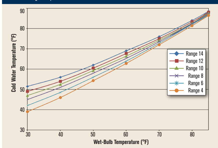
FIGURE 1 Cooling tower performance.
