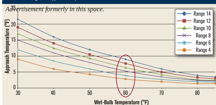
FIGURE 2 Cooling tower approach temperature.
