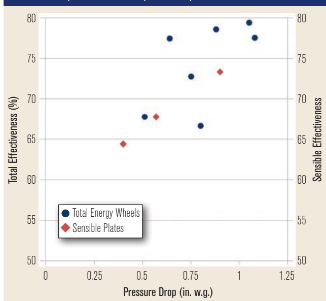
FIGURE 2 Sample effectiveness vs. pressure drop.
