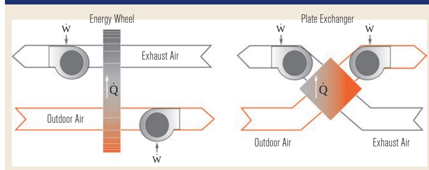
FIGURE 1 Energy exchanged between airstreams for more work by the fans.
